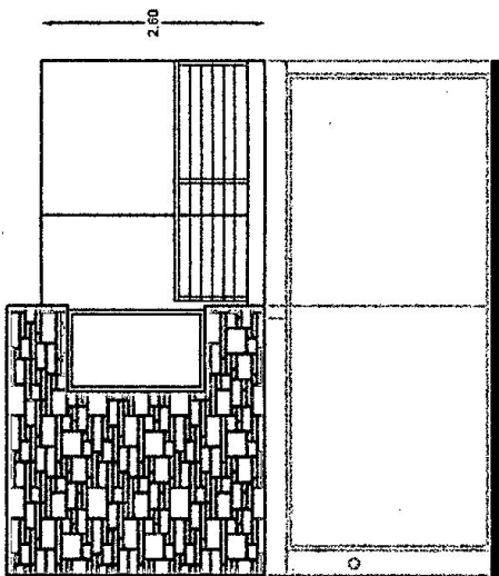
FACHADA PRINCIPAL
